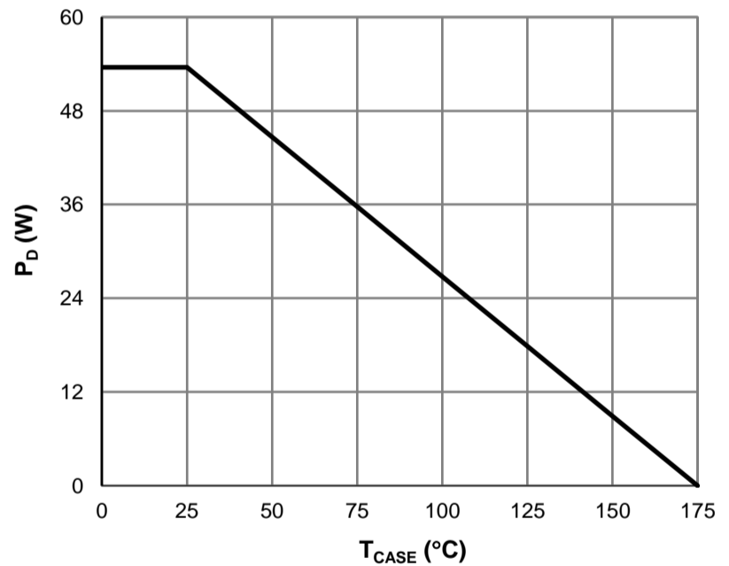
Figure 10: Power De-rating
